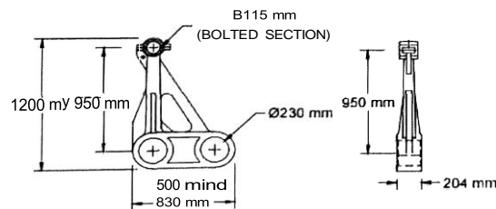
DETAIL OF DOUBLE CAVITY STANCHION WITH SEAMLESS BOTTOM SECTION
