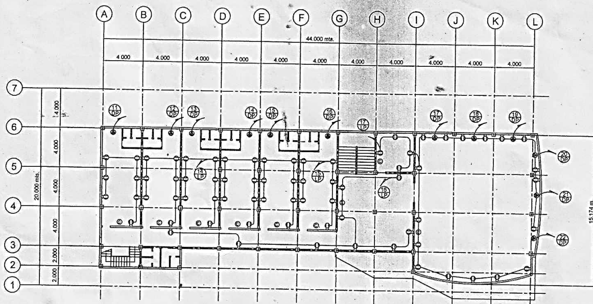
E SECOND FLOOR POWER LAYOUT 1 D SCALE 1:200 MTS.
