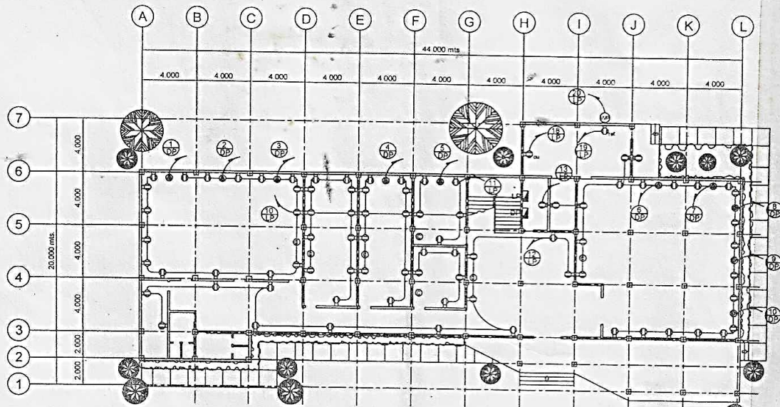
E GROUND FLOOR POWER LAYOUT 1 C SCALE 1:200 MTS
