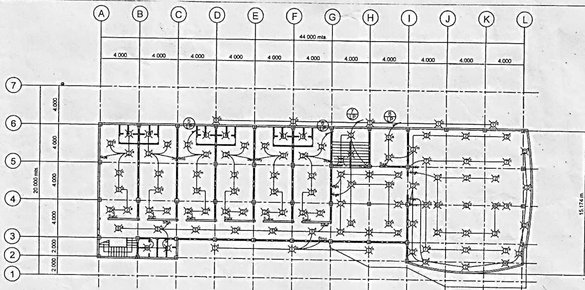
E SECOND FLOOR LIGHTING LAYOUT 1 B SCALE 1:200 MTS.
