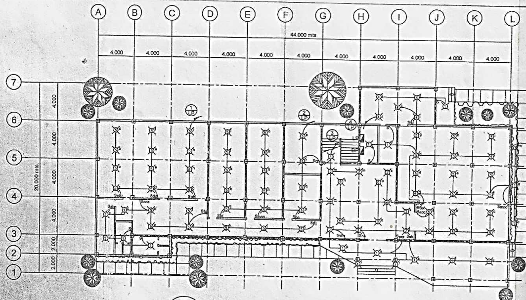
E GROUND FLOOR LIGHTING LAYOUT 1 A SCALE 1:200 MTS
