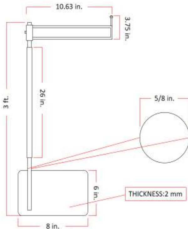
Rudder Assembly
